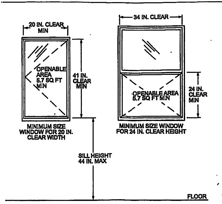
Figure R310.2.1 EMERGENCY ESCAPE AND RESCUE WINDOW
