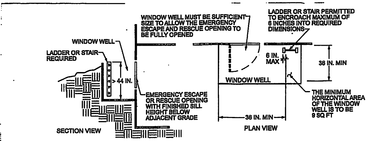
Figure R310.2.3 WINDOW WELLS
